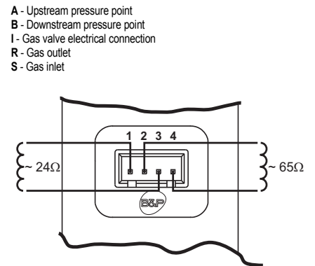
fig. 12 - Gas valve connection
